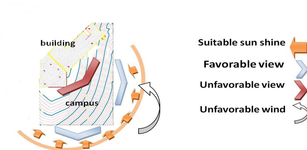
Fig. 6: Climate analysis
